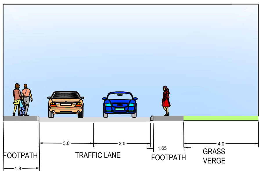
EXISTING CROSS SECTION AT A-A
