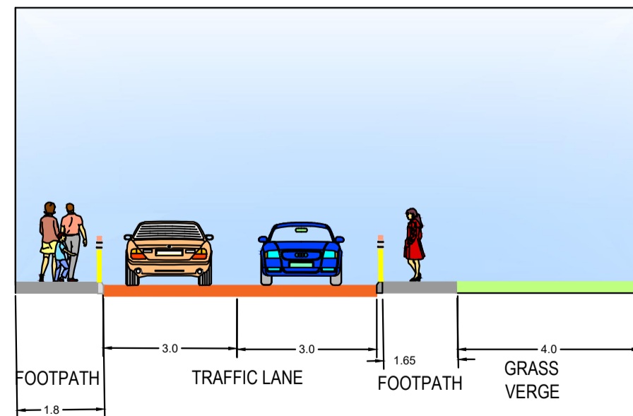
PROPOSED SECTION AT A-A
